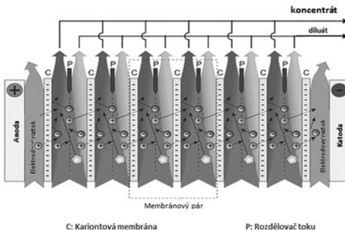
Obr. 5.6 Princip PED s CM [10]
